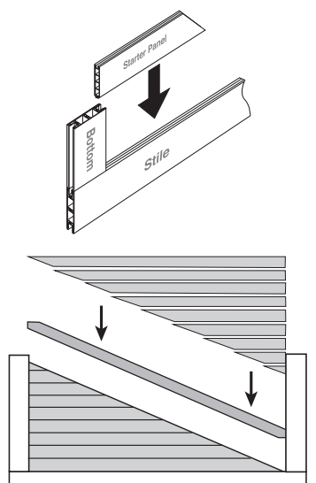
Figure 8 Starter Panel
